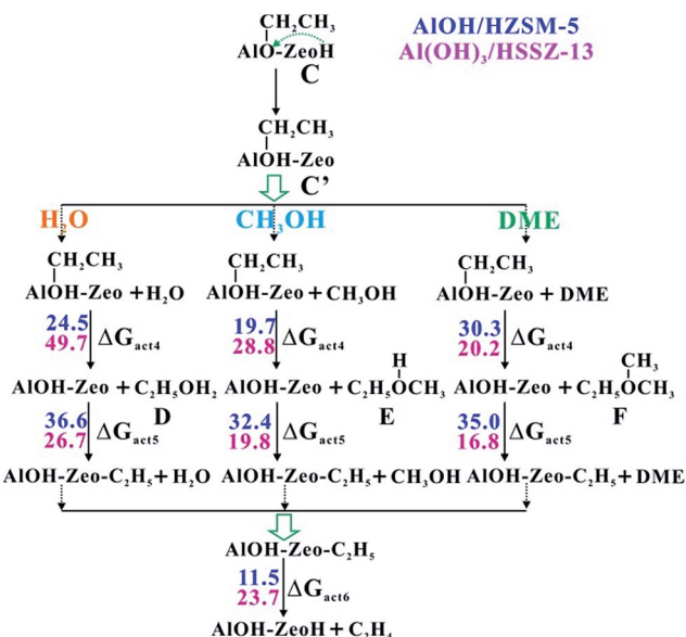
Fig. 4 The proposed route for ethene formation from intermediate C over AIOH/HZSM-5 and Al(OH) 3 /HSSZ-13 (see Scheme S2†). The Gibbs free energy barriers ( \Delta G_{\text{act}} , in kcal mol -1 ) for each elementary step at 573 K have been listed (D, represents the protonated ethanol; E, represents the protonated CH 3 CH 2 OCH 3 ; F, represents CH 3 CH 2 -O + (CH 3 ) 2 oxonium).
