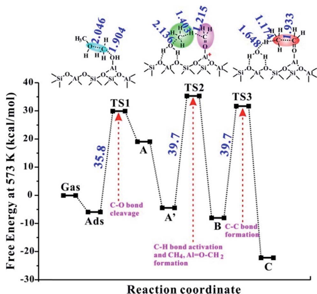
Fig. 3 The reaction Gibbs free energy profile of the direct formation of the C–C bond following the newly proposed mechanism (see Scheme 1) at the \text{Al(OH)}_2^+/\text{BAS} site over ZSM-5 zeolite at 573 K. The detailed reaction routes and definition of the abbreviations are shown Scheme 1. The main geometric parameters of the TS are given in Å.
