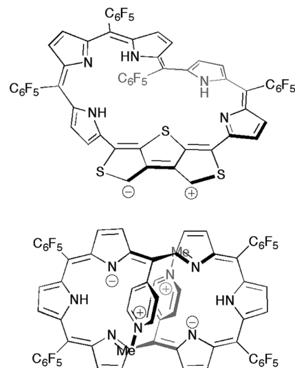
Fig. 7 Possible zwitterionic structures of [28]hexaphyrin 5 (top) in comparison to the methylpyridinium-substituted analogue (bottom).
