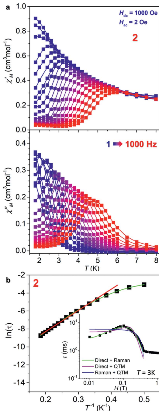
Fig. 4 (a) The in-phase ( \chi' ) and out-of-phase ( \chi'' ) components of the ac susceptibilities as a function of T of 2 in 1000 Oe dc field at different time frequencies (1–1000 Hz). (b) Natural logarithm of the relaxation time \ln \tau as a function of the inverse temperature T^{-1} . The straight red line is a fit of the 12 points at highest temperatures to the Arrhenius law \ln \tau = \ln \tau_0 + U_{\text{eff}}/k_{\text{B}}T . The curved green line is the best fit to the sum of the direct and Raman processes (see ESI†). Inset: field dependence of the magnetic relaxation times at 3 K for 2 and its approximation by the different models assuming two magnetic relaxation mechanisms, where only the sum of the direct and Raman processes gives a good fit.
