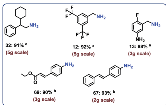
Fig. 7 Representing the practical utility of the cobalt-catalyzed hydrogenation protocol for gram scale reactions. Reaction conditions: a 3–5 g nitrile, 25 mg catalyst (3.8 mol% Co) for each 0.5 mmol substrate, 25 bar H 2 , 5 bar NH 3 , 120 °C, 20–60 mL toluene 16 h, isolated respective hydrochloride salts. b 2–3 g nitroarene 25 mg catalyst (3.8 mol% Co) for each 0.5 mmol substrate, 40 bar H 2 , 120 °C, 20–40 mL THF–H 2 O (1 : 1), 20 h, isolated yields.
