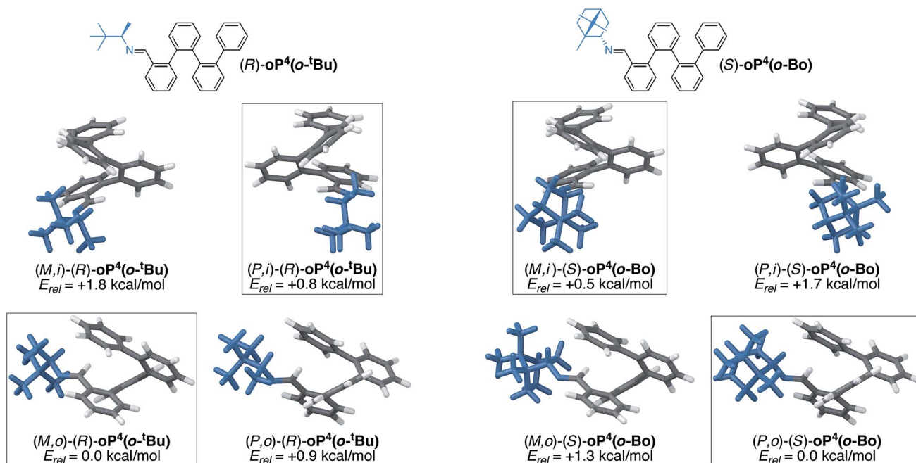
Fig. 13 Optimized M and P geometries and their relative stabilities of inward- ( i ) and outward-facing ( o ) conformers for ( R )- oP 4 (o- t Bu) (left) and ( S )- oP 4 (o-Bo) (right) (PCM(CHCl 3 )/B97-D/TZV(2d,2p)). Boxes indicate the favored conformers for each imine orientation.
