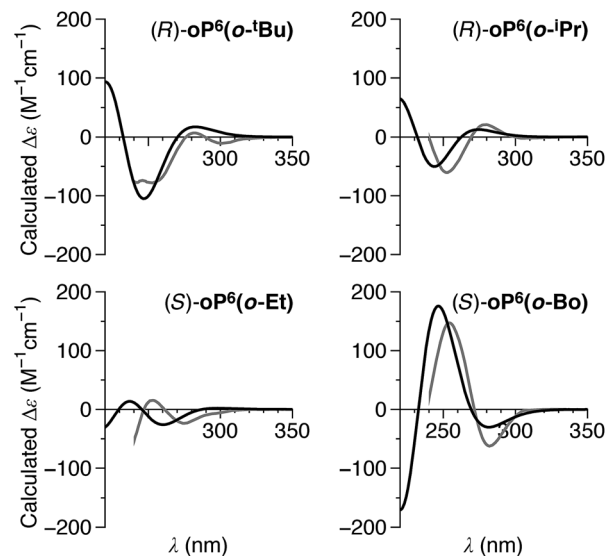
Fig. 12 Predicted CD spectra of (R)\text{-oP}^6(\text{o-t-Bu}) , (R)\text{-oP}^6(\text{o-i-Pr}) , (S)\text{-oP}^6(\text{o-Et}) , and (S)\text{-oP}^6(\text{o-Bo}) (black). Experimental spectra (gray) were scaled identically ( i.e. , relative intensities can be directly compared). The simulated spectra were generated by estimating the contributions of the calculated spectra for (M)\text{-oP}^6(\text{o-H}) (Fig. 11) using the conformer populations and diastereomeric excesses determined by ^1\text{H} NMR (Table 2).
