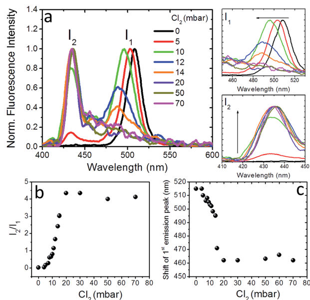
Fig. 4 (a) Normalized fluorescence spectra of, 0.5 mm thick, \text{PDMS}:\text{CsPbBr}_3 NCs nanocomposite layers upon exposure to different partial \text{Cl}_2 pressures. The corresponding evolution of the initial peak with intensity I_1 (top) and of the peak that emerges after chlorine treatment with intensity I_2 , (bottom) are shown on the right. (b) Fluorescence intensity ratio, I_2/I_1 , and (c) spectral shift of the first emission peak, as a function of the partial pressure of \text{Cl}_2 gas.
