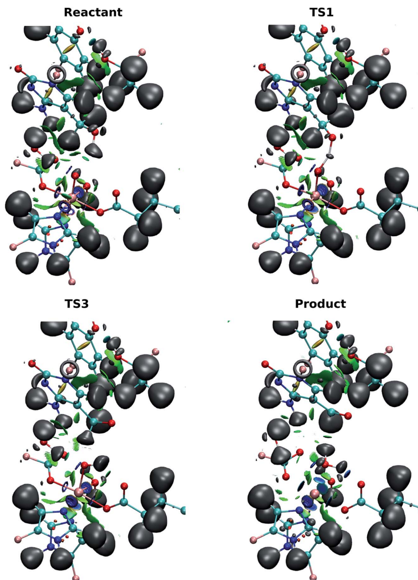
Fig. 7 ELF and NCI surfaces for the active site of (a) reactant; (b) TS1; (c) TS3; (d) product in the wild-type TET2-5hmC/fC complex. The isovalue for ELF and NCI is 0.5. For the NCI surfaces, the color scale is chosen so that blue indicates relatively strong attraction, green indicates relatively weak interaction, and red indicates relatively strong repulsion in the region of non-covalent interactions. The MM region is not shown for clarity.
