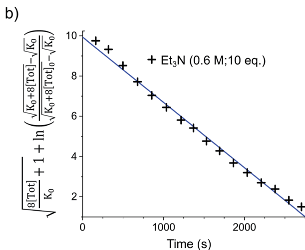
Fig. 3 (a) Solutions of 1 (0.03 mmol) in d_8 -toluene (0.5 mL) under \text{H}_2 (4 bar) containing various base concentrations were prepared. When the stannylene concentration, [\text{Tot}] , is plotted against the normalised timescale t \cdot [\text{Et}_3\text{N}]^1 , all traces overlap, confirming the order in base to be one. (b) Linearised rate data for a similar solution of 1 (0.03 mmol) in d_8 -toluene (0.5 mL) under \text{H}_2 (4 bar) containing \text{Et}_3\text{N} (0.6 M; 10 eq.).
