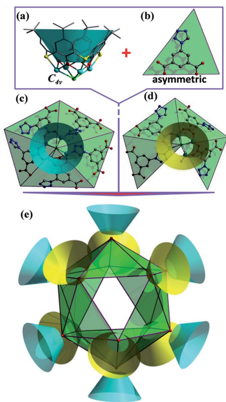
Fig. 1 The structure of the M_{48} ( M = Co, Ni ) cage cluster determined by X-ray crystallography: (a) representations of the [(M_4\text{-TC4A})Cl] SBU with an approximate C_{4v} symmetry (all hydrogen atoms omitted for clarity), (b) the asymmetric 5-(1 H -tetrazol-1-yl)isophthalate ( L^{2-} ) ligand, (c) SBU-1 with five L^{2-} ligands, (d) SBU-2 with four L^{2-} ligands and (e) the M_{48} cage cluster showing the merohedral icosahedral arrangement of 12 [(M_4\text{-TC4A})Cl] units. Color code: M turquoise, S yellow, Cl green, O red, N blue, C gray, TC4A in SBU-1 turquoise and in SBU-2 yellow, and merohedral icosahedron green.
