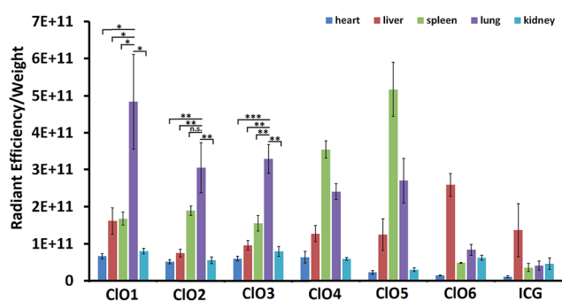
Fig. 4 The ratio of radiant efficiency to the organ weight of mice intravenously injected with ClO1–ClO6 and ICG. ( n = 3 ; * P < 0.05 ; ** P < 0.01 ; *** P < 0.001 ; n.s., P > 0.05 ; t test, double-tailed).
