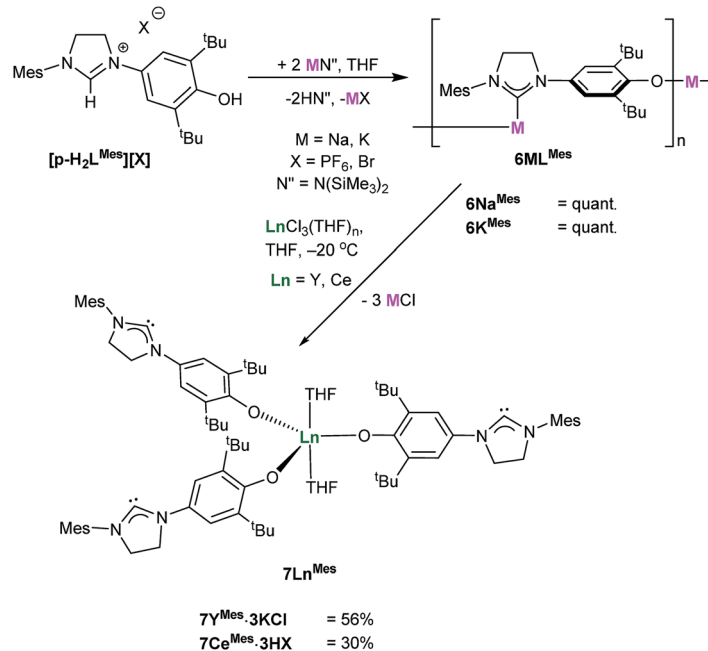
Scheme 7 Reaction to target the para -ligand adducts 7\text{Ln}^{\text{Mes}} (Ln = Y, Ce).
