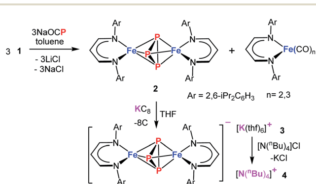
Scheme 1 Synthesis of molecular precursor 2 and its reactivity.
