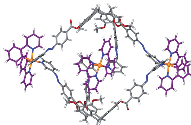
Fig. 6 Energy-minimized structure of [\text{Ir}(\text{ppy})_2]_3(\text{L}2)_2]^+ .
