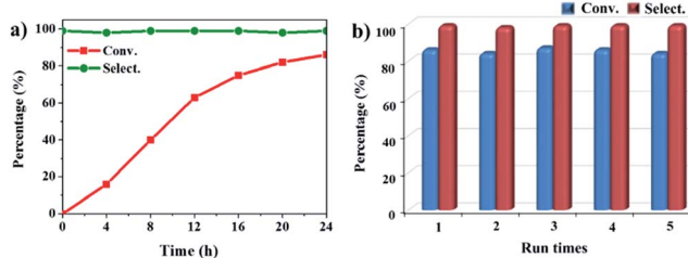
Fig. 5 (a) The kinetic curve and (b) recyclability for Pd–Cu@HO-NPC in the oxidation reaction of indane. Reaction conditions: indane (8.77 mmol), catalyst ([Pd] = 0.2 mol%), air flow (5 mL min -1 ), 120 °C and 24 h.
