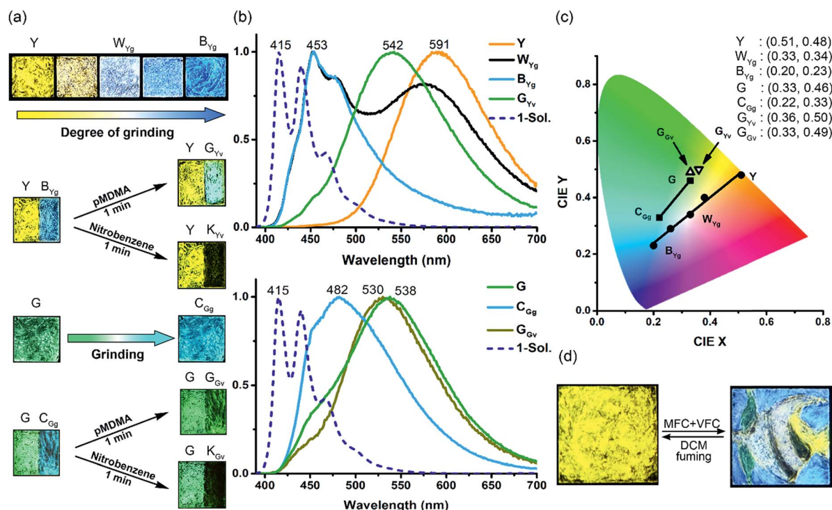
Fig. 3 MFC and VFC of the Y and G powder films of 1 : (a) photographs of the fluorescence colour ( \lambda_{\text{ex}} = 365\text{ nm} ); (b) the corresponding normalized fluorescence spectra ( \lambda_{\text{ex}} = 380\text{ nm} ); (c) the corresponding coordinates and positions on the CIE chromaticity diagram; (d) multi-colour fluorescence patterning of “an angelfish and an aquatic plant” on a powder film ( 1.5\text{ cm} \times 1.5\text{ cm} ) of the Y form. See Fig. S8† for detailed drawing and patterning procedures and intermediate stages. The fluorescence spectrum of 1 in DCM (blue dashed line) is included in (b) for comparison.
