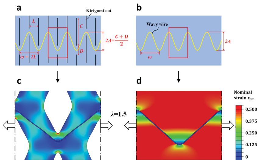
Fig. 5 Kirigami film–wavy wire structure enhancing effective wire adhesion. (a) Design of the kirigami film–wavy wire structure, where the wire follows a sinusoidal shape with wavelength \omega = 2L and amplitude A = (C + D)/4 . (b) The same wavy wire is bonded on the corresponding continuous film. (c) Distribution of nominal strain \epsilon_{xx} in the kirigami film–wavy wire structure under applied stretch \lambda = 1.5 . (d) Distribution of nominal strain \epsilon_{xx} in the corresponding continuous film under applied stretch \lambda = 1.5 .
