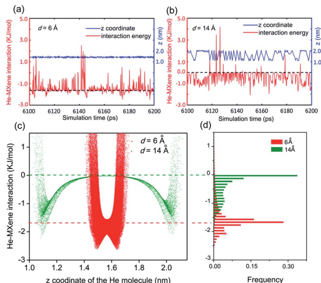
Fig. 2 The time series of a helium molecule's z coordinate (blue), interaction energy with MXene sheets (red), which diffuses in anhydrous MXene nanogalleries with interlayer distance d = 6 Å (a) and 14 Å (b). (c) The He–MXene interaction energy– z coordinate scatter plot of a He molecule diffusing in d = 6 Å (red) or 14 Å (olive) anhydrous MXene nanogalleries. (d) The normalized distribution of He–MXene interaction energy for a He molecule diffusing in d = 6 Å (red) or 14 Å (olive) anhydrous MXene nanogalleries.
