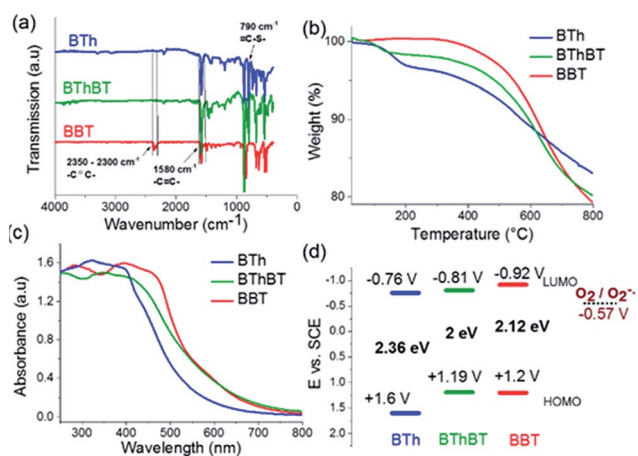
Fig. 3 (a) FTIR and (b) TGA spectra of the materials under a \text{N}_2 atmosphere with a heating rate of 10\text{ }^{\circ}\text{C min}^{-1} ; (c) UV/vis DR spectra and (d) energy band structures of the as synthesized CMPs and the \text{O}_2/\text{O}_2^{\cdot-} couple.
