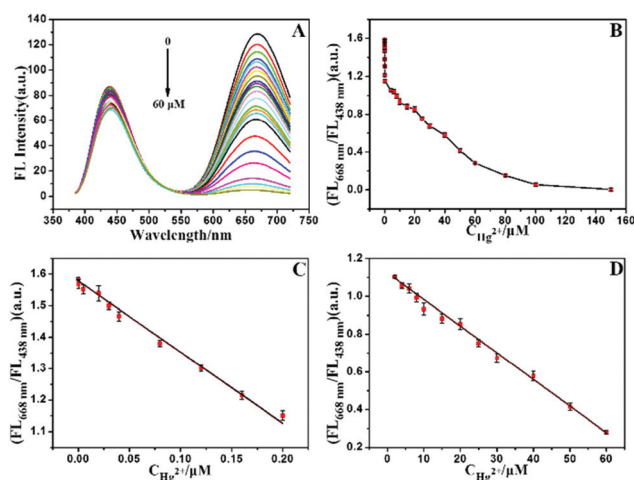
Fig. 2 (A) Fluorescence emission spectra of AuNCs/MIL-68(In)-NH 2 /Cys in the presence of Hg 2+ with different concentrations (0, 2 × 10 -4 , 5 × 10 -3 , 0.02, 0.03, 0.04, 0.08, 0.12, 0.16, 0.2, 0.2, 4, 6, 8, 10, 15, 20, 25, 30, 40, 50 and 60 μM). (B) Plot of the fluorescence intensity ratio (FL 668 nm /FL 438 nm ) versus the concentration of Hg 2+ . (C) The linear relationship between FL 668 nm /FL 438 nm and the concentration of Hg 2+ ranging from 20 pM to 0.2 μM. (D) The linear relationship between FL 668 nm /FL 438 nm and the concentration of Hg 2+ ranging from 0.2 μM to 60 μM. The error bars represent the standard deviation of three measurements (λ ex = 370 nm, slit: 5/5 nm).
