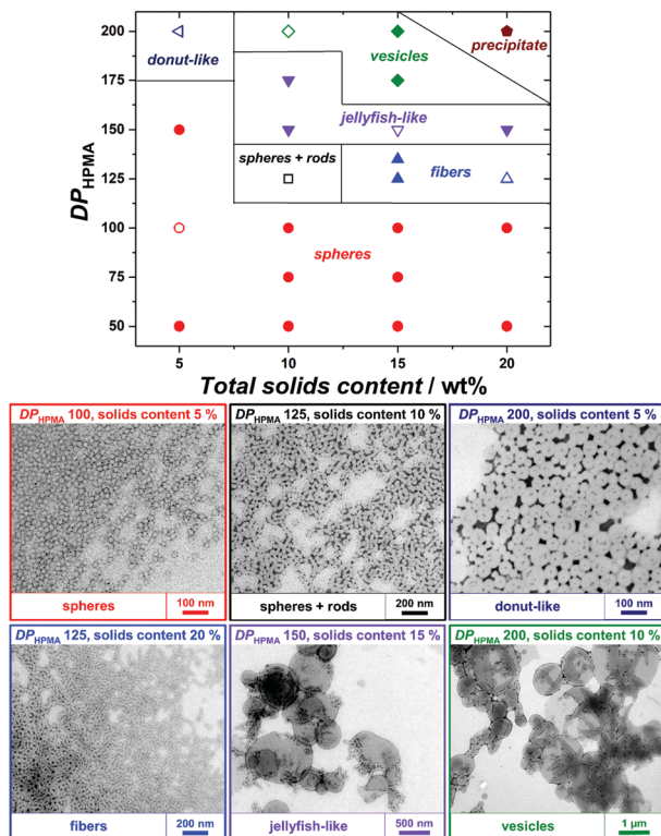
Fig. 1 (top) Phase diagram for RAFTPIISA of HPMA using PETox-CTA M4 as macroRAFT agent and (bottom) TEM images of representative samples (empty symbols from above). Larger TEM images are provided as Fig. S25 (ESI † ).
