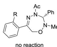
Scheme 22 Cu(II)-Catalyzed asymmetric 1,3-dipolar [4+3] cycloaddition and kinetic resolution of azoalkenes with azomethine imines.
