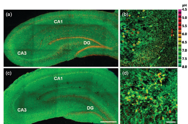
Fig. 43 Pseudocolored ratiometric TPM images ( I_{\text{green}}/I_{\text{IR}} ) of a rat hippocampal slice stained with 30 \mu\text{M} (a and b) 28 and (c and d) 27a . (a and c) 120 \mu\text{m} TPM images along the z-direction at depths of approximately 90\text{--}180 \mu\text{m} were accumulated to visualize the overall pH distribution with 10\times magnification. (b and d) Higher magnification images ( 63\times ) in the regions of DG. Excitation wavelength is 740 nm. Scale bars are (a and c) 300 \mu\text{m} and (b and d) 47 \mu\text{m} . Copyright 2013 American Chemical Society.
