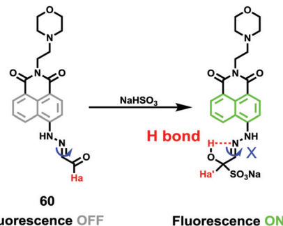
Scheme 46 Fluorescent probe 60 for SO 2 .
