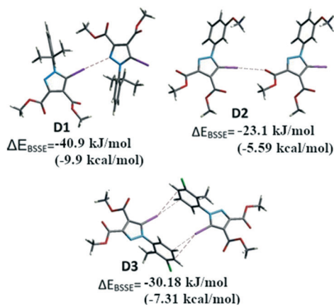
Fig. 10 The dimers D1–D3 formed by I...N, I...O and I... \pi interactions respectively.
