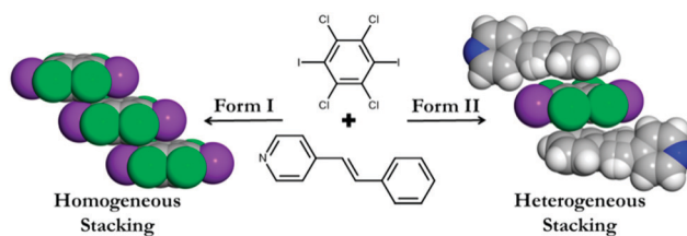
Scheme 1 The \pi - \pi stacking arrangement within the two polymorphs of (C 6 I 2 Cl 4 )·2(4-SB).
