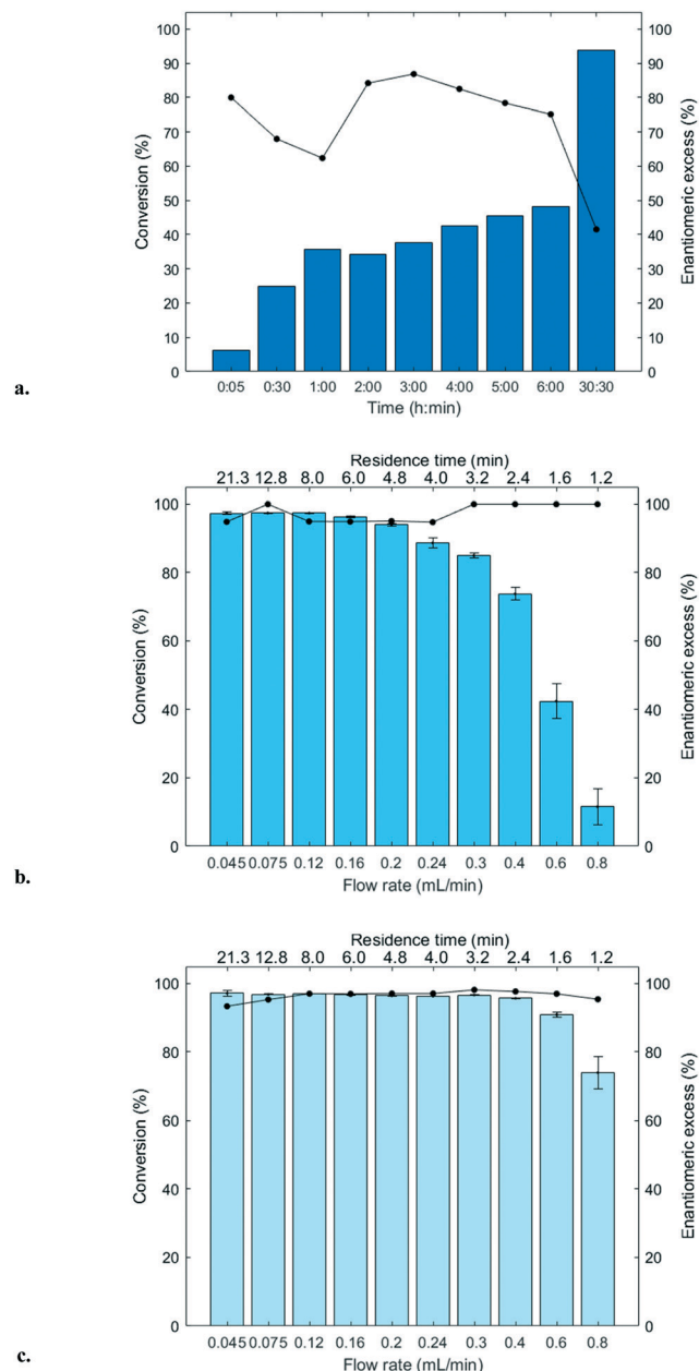
Fig. 3 ( S )-Mandelonitrile (( S )-2) synthesis reaction: a. HbHNL -MCF-APT (50 mg; 2.5 mg total protein; 150 U), 2 mL HCN in MTBE (1.5–2 M) saturated with citrate phosphate buffer (pH 5.0, 50 mM), benzaldehyde (1) 100 \mu L (1 mmol), ISTD 1 (1,3,5-trisopropylbenzene) 27.5 \mu L (0.1 mmol), shaken at 1000 rpm at room temperature (18–22 ^{\circ} C) under nitrogen atmosphere, conversion (bars)/enantiomeric excess (black line) vs. time (h). HbHNL -silica monolith (11.3 mg total protein; 1120 U per monolith) conversion (bars)/enantiomeric excess (black line) (%) vs. flow rate (mL min −1 )/residence time (min). c. MeHNL -silica monolith (17.4 mg total protein; 1310 U per monolith) conversion (bars)/enantiomeric excess (black line) vs. flow rate (mL min −1 )/residence time (min). Flow rate is total of two pumps. Pump 1 pumps benzaldehyde (1) in MTBE (0.50 M, containing 0.066 mM ISTD 1) and pump 2 pumps HCN in MTBE (1.5–2.0 M, containing 0.066 mM ISTD 2 saturated with citrate phosphate buffer (pH 5.0, 50 mM)). Error bars indicate the standard deviation based on triplicate ( n = 3) HPLC samples (see Experimental section).
