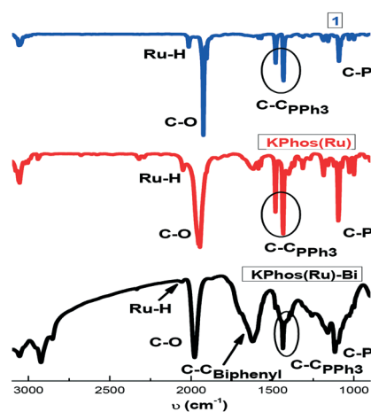
Fig. 2 FTIR spectra of the parent Ru-complex and knitted Ru(PPh 3 ) 3 -polymers.
