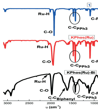
Fig. 2 FTIR spectra of the parent Ru-complex and knitted \text{Ru(PPh}_3\text{)} -polymers.
