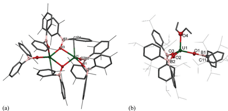
Fig. 1 Displacement ellipsoid drawing of the molecular structure of (a) 1^m and (b) 1^t \cdot Et_2O . The hydrogen atoms are omitted and the mesityl and triisopropylphenyl groups are depicted as wireframe and capped sticks for clarity. The thermal ellipsoids are displayed at 50% probability.
