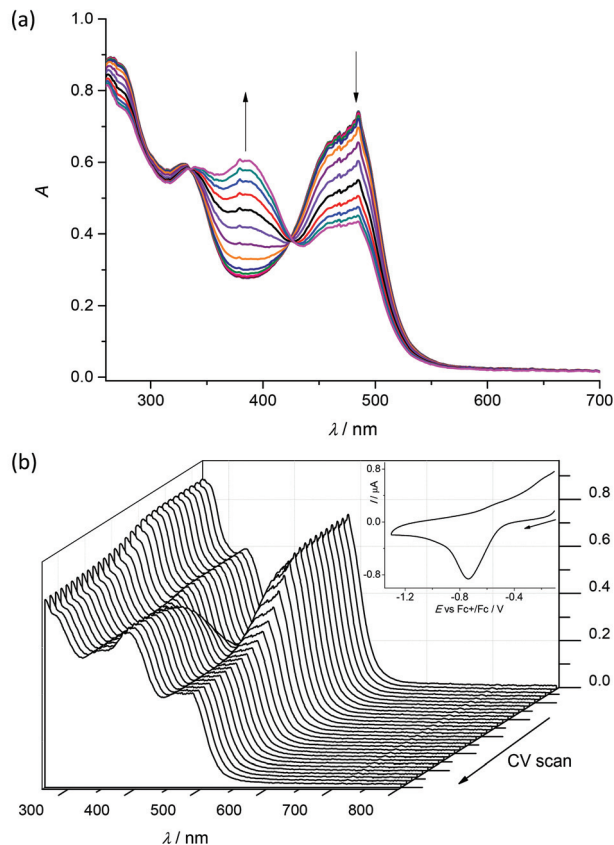
Fig. 7 In situ UV-vis-NIR spectroelectrochemistry for 1 in DMSO/ n\text{Bu}_4\text{NPF}_6 (scan rate of 10\text{ mV s}^{-1} , Pt-microstructured honeycomb working electrode): (a) evolution of UV-vis spectra in 2D projection in forward scan in the region of the first reduction peak; (b) UV-vis spectra detected simultaneously upon the cyclic voltammetric scan in 3D projection (Inset: The corresponding cyclic voltammogram).
