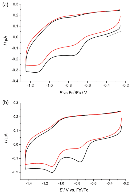
Fig. 6 Cyclic voltammograms of (a) 1 and (b) 4 in DMSO/ n\text{Bu}_4\text{NPF}_6 at scan rate of 100\text{ mV s}^{-1} at GC working electrode (black traces represent the first scan, while red traces the second scan).
