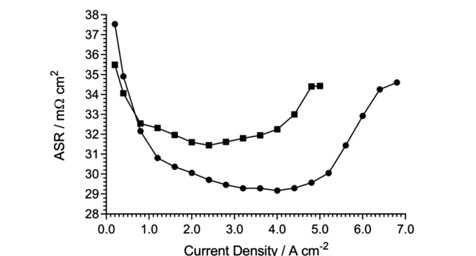
Fig. 6 Comparison of HDPE-AEM-containing \text{H}_2/\text{O}_2 AEMFC performances at 80^\circ\text{C} with cathodes containing a Pt/C catalyst (40 wt% Pt, 0.4 \text{ mg cm}^{-2} Pt loading) and a Ag/C catalyst (40 wt% Ag, 0.85 \text{ mg cm}^{-2} Ag loading). All other MEA and cell test parameters as in Fig. 4. 4 ASRs were measured using the 850E tester's internal current interrupt method.
