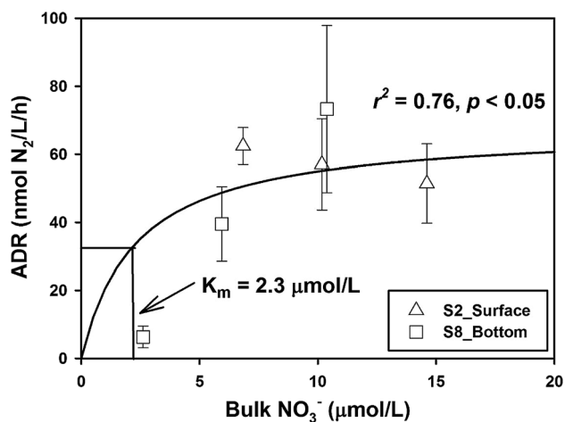
Fig. 2 Response of apparent denitrification rate (ADR) with manipulated \text{NO}_3^- concentration at Stations S2 and S8. The solid line is fitted according to the Michaelis–Menten kinetics. K_m represents the half-saturation constant of \text{NO}_3^- demand.
