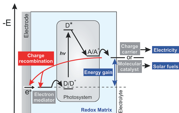
Fig. 1 Energy level diagram and schematic illustration of reactions in a biophotocathode based on photosynthetic proteins. The light-induced charge separation at the photosynthetic protein triggers the electron transfer chain. The electron mediator refills the hole at the donor site ( D/D^+ ) of the photosystem and a charge carrier or a molecular catalyst recovers the electron from the acceptor site ( A/A^+ ). The electron mediator shuttles the charge from the electrode while the charge carrier can be used to generate electricity or the molecular redox catalyst catalyzes reactions for solar fuel generation. The energy gained from light leads to a potential difference between the electron mediator and the charge carrier defines the driving force for charge recombination of the charge carrier at the mediator or at the electrode.
