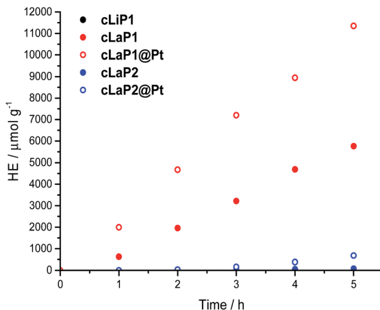
Fig. 4 Hydrogen evolution of cLiP1, cLaP1 and cLaP2 as well as cLaP1@Pt and cLaP2@Pt from a \text{H}_2\text{O}/\text{TEA}/\text{MeOH} mixture under broadband irradiation (300 W Xe light source, \lambda > 295 nm).
