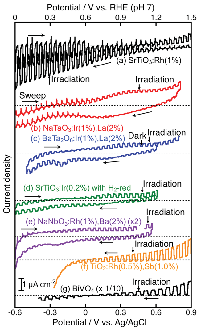
Fig. 5 Current vs. potential curves of (a) \text{SrTiO}_3\text{:Rh(1\%)} , (b) \text{NaTaO}_3\text{:Ir(1\%),La(2\%)} , (c) \text{BaTa}_2\text{O}_6\text{:Ir(1\%),La(2\%)} , (d) \text{SrTiO}_3\text{:Ir(0.2\%)} with \text{H}_2 reduction, (e) \text{NaNbO}_3\text{:Rh(1\%),Ba(2\%)} , (f) \text{TiO}_2\text{:Rh(0.5\%),Sb(1.0\%)} , and (g) \text{BiVO}_4 . Electrolyte: 0.1 \text{ mol L}^{-1} \text{ K}_2\text{SO}_4 aqueous solution (pH 7, phosphate buffer was added if necessary), light source: 300 W Xe lamp ( \lambda > 420 \text{ nm} ).
