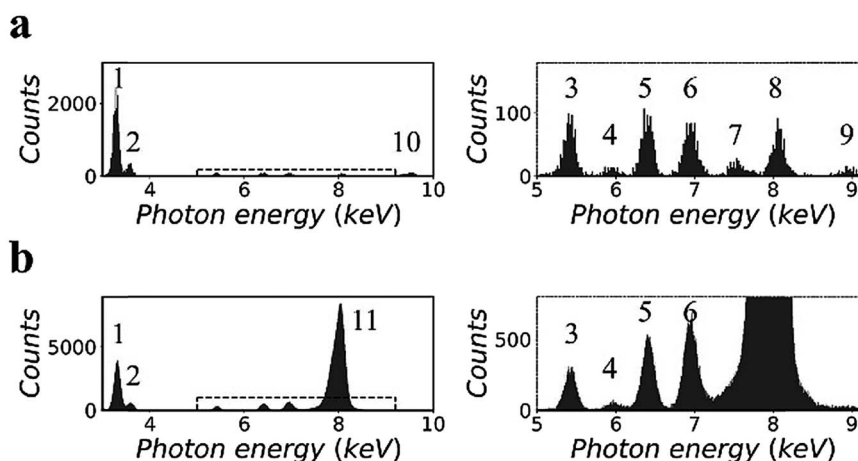
Fig. 2 X-ray fluorescence spectra of the lithium borate pellet that includes 100 ppm chromium, iron, cobalt, and copper: (a) measured in the synchrotron polarized experiment and (b) measured in the laboratory unpolarized experiment. Details of spectra were enlarged and attached on the right side.
