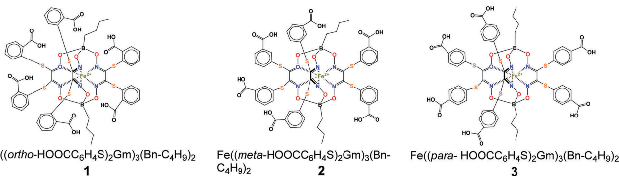
Scheme 1 Chemical drawings of the hexacarboxyphenylsulfide iron(II) clathrochelates under study.
