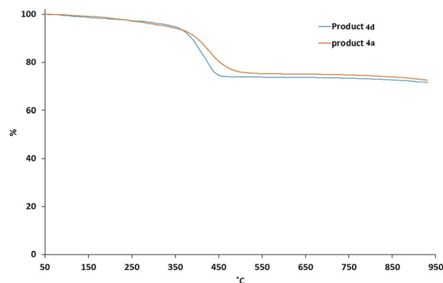
Fig. 6 TGA of the mixed ligand-stabilized titanium dioxide nanorods 4a , with the relatively short hexyl spacer group, and the corresponding mixed ligand-stabilized, titanium dioxide nanorods 4d , with a longer undecyl spacer group between the TiO 2 nanorod and the photo-reactive coumarin endgroup.
