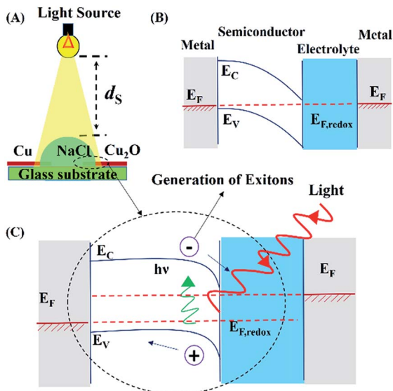
Fig. 1 Image (A) shows the experimental set-up in which a droplet of aqueous solution of NaCl was dispensed between the Cu and Cu 2 O electrodes before being illuminated by a light source from the top. The electrodes were placed on a glass slide as shown. Images (B) and (C) schematically show the band diagrams of the configuration in the absence and presence of the photo-excitations, respectively. The notations E_F , E_C , and E_V indicate the Fermi level and energy levels for the conduction and valence bands, respectively. The notation E_{F,redox} denotes the Fermi level in the electrolyte.
