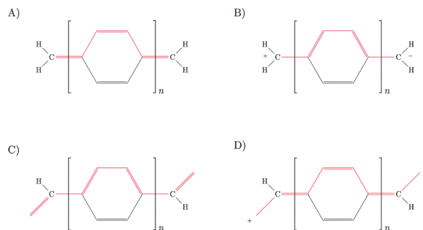
Fig. 7 Resonant forms of \mathbf{pX2} structures: (A) trivial , (B) topological and \mathbf{pP} structures: (C) trivial , (D) topological . The main polyacetylene structures are depicted in red and the bridging ethylene units in black.
