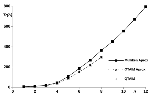
Fig. 6 Trace of the LT calculated for the methylene carbons with the Mulliken and QTAIM atomic partitionings, using eqn (11) and (12) vs. number of phenyl units, n , in the \mathbf{pX2} chains.
