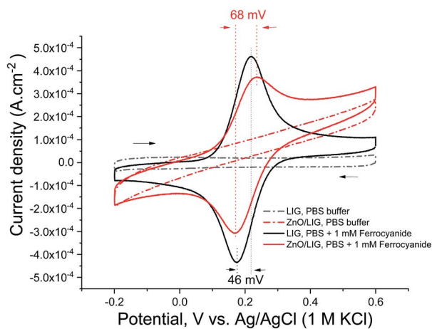
Fig. 8 CVs of LIG reference (black lines) and ZnO/LIG composite (red lines) at 100 \text{ mV s}^{-1} . The measuring solutions are PBS only (dashed lines) and PBS with 1 mM ferrocyanide (solid lines).
