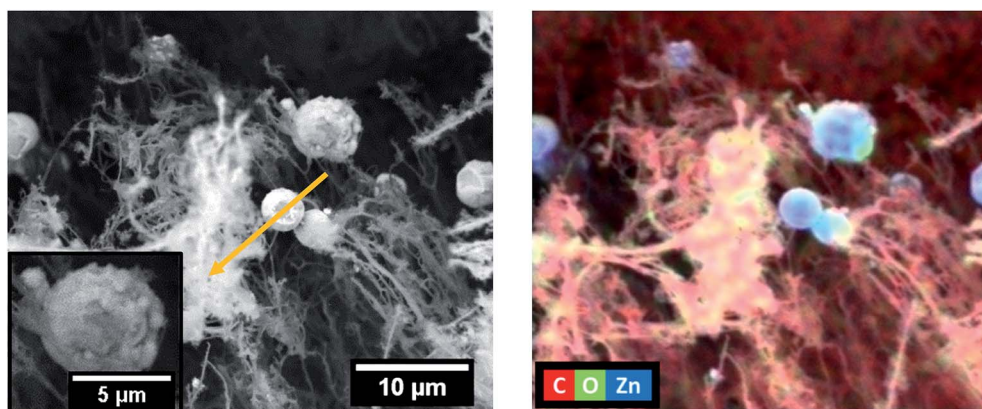
Fig. 3 SEM image of a sample produced with ~24 W, v = 350 \text{ mm s}^{-1} , d = 0.075 \text{ mm} and focused conditions (left) and EDS mapping of the correspondent region (right).
