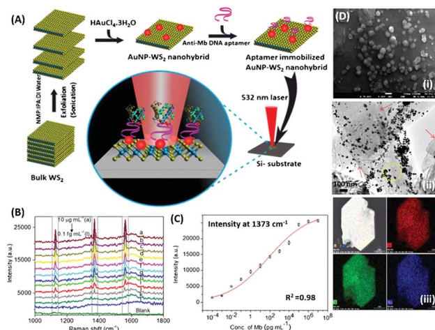
Fig. 7 (A) Schematic representation of the synthesis of the WS 2 -AuNP SERS-active nano-hybrid and its utilisation in the detection of myoglobin. (B) Raman spectra showing the increase in signal intensity in response to various concentration of myoglobin. (C) Fitting of signal intensity at 1373 cm -1 . (D) Electron micrographs of the nano-hybrid and its corresponding elemental mapping. Reprinted with permission from ref. 98. Copyright (2018) Springer Nature.
