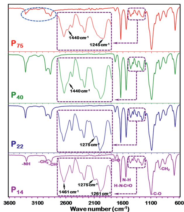
Fig. 7 FTIR spectra of \text{P}_{14} , \text{P}_{22} , \text{P}_{40} and \text{P}_{75} PEBAX membranes. Inset spectra represent the variation in vibrational peaks in the range of 1200 – 1500 \text{ cm}^{-1} .
