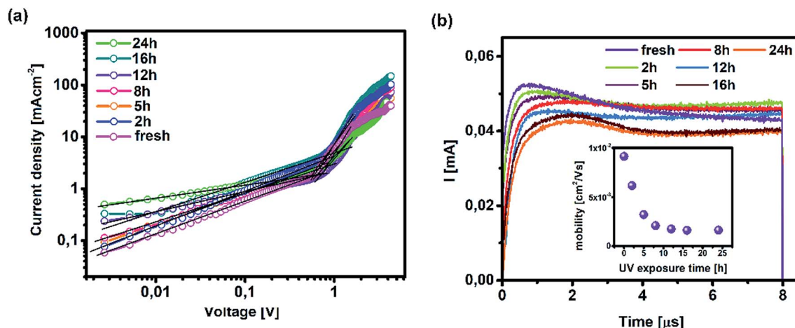
Fig. 6 (a) Dark J–V current traces for hole-only devices (ITO/PTAA/MAPI/Au) upon UV exposure and (b) photo-CELIV transients of measured inverted planar solar cells (ITO/PTAA/MAPI/PC 60 BM/PFN/Ag) and corresponding mobilities (inset).
