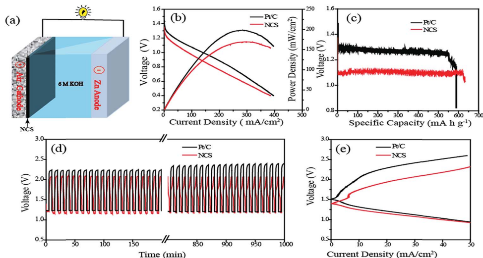
Fig. 6 (a) Schematic structure of the Zn–air battery, (b) I – V polarization curves of the battery by using NCS and Pt/C as the cathode materials, (c) typical discharge curves of the Zn–air battery under continuous discharge until complete consumption of Zn, (d) charge–discharge cycles performed at a current density of 10 \text{ mA cm}^{-2} and (e) charging and discharging polarization ( I – V ) plots of the rechargeable Zn–air battery.
