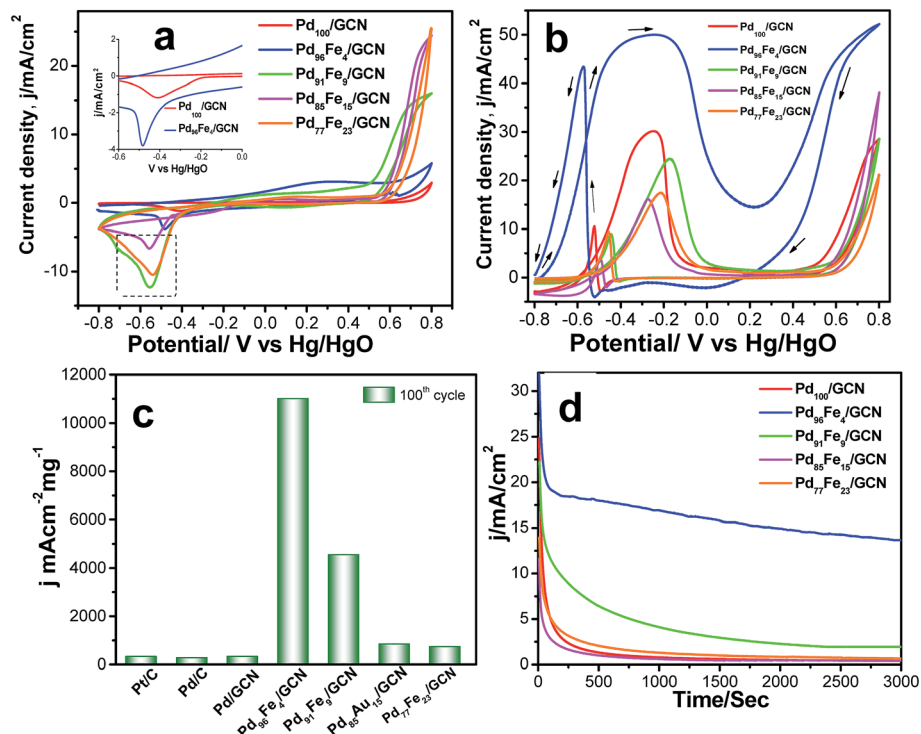
Fig. 7 (a) CVs of the Pd 100 /GCN, Pd 96 Fe 4 /GCN, Pd 91 Fe 9 /GCN, Pd 85 Fe 15 /GCN, and Pd 77 Fe 23 /GCN nanoalloys in 0.5 M KOH at a scan rate of 50 mV s -1 . (b) CVs for the electrocatalytic oxidation of 0.5 M ethanol at the 100 th cycle by Pd 100 /GCN (red solid line), Pd 96 Fe 4 /GCN (blue solid line), Pd 91 Fe 9 /GCN (green solid line), Pd 85 Fe 15 /GCN (pink solid line), and Pd 77 Fe 23 /GCN (orange solid line) nanoalloys at a scan rate of 50 mV s -1 in 0.5 M KOH. (c) Comparative values of mass activity of Pd/C, Pd/C, Pd 100 /GCN, Pd 96 Fe 4 /GCN, Pd 91 Fe 9 /GCN, Pd 85 Fe 15 /GCN, and Pd 77 Fe 23 /GCN electrodes for ethanol oxidation in alkaline medium. (d) Chronoamperometric curves for the ethanol oxidation at a constant potential of -0.22 V vs. Hg/HgO on Pd 100 /GCN, Pd 96 Fe 4 /GCN, Pd 91 Fe 9 /GCN, Pd 85 Fe 15 /GCN, and Pd 77 Fe 23 /GCN electrodes.
