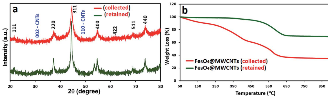
Fig. 5 (a) XRD patterns and (b) TGA curves for \text{Fe}_3\text{O}_4 @MWCNT exiting (red) and retained (green) in the quartz tube, processed in the VFD (optimised parameters) operating at 8.5k rpm rotational speed, with the concentration of the as received MWCNTs at 0.08\text{ mg mL}^{-1} (DMF), tilt angle 45^\circ , flow rate 0.45\text{ mL min}^{-1} , and laser power 250 mJ.
