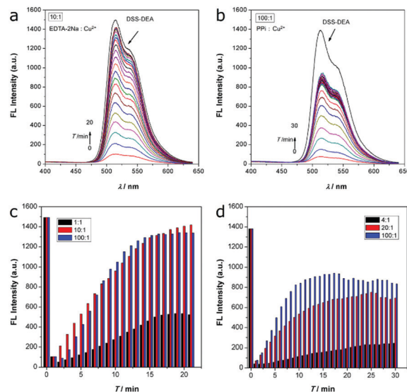
Fig. 5 (a) EDTA-2Na induced fluorescence recovery in 20 minutes (EDTA-2Na: Cu^{2+} 10:1). (b) PPI induced fluorescence recovery in 30 minutes (PPI: Cu^{2+} 100:1). (c) The recovery trend of the EDTA-2Na at different EDTA-2Na/ Cu^{2+} ratios induced fluorescence recovery of the DSS-4-DEA/ Cu^{2+} complex. (d) The recovery trend of the PPI at different PPI/ Cu^{2+} ratios induced fluorescence recovery of the DSS-4-DEA/ Cu^{2+} complex.
