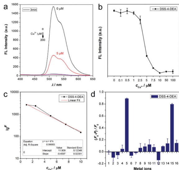
Fig. 4 (a) Cu^{2+} (0–200 \mu M ) induced fluorescence quenching of DSS-4-DEA (100 \mu M ) after 3 minutes of stabilization. (b) Finely measured Cu^{2+} (0.1–100 \mu M ) induced fluorescence quenching of the DSS-4-DEA. (c) Fluorescence intensity against the concentration of Cu^{2+} . (d) Metal ion induced fluorescence quenching of the DSS-4-DEA (1 Ca^{2+} , 2 Cd^{2+} , 3 Co^{2+} , 4 Cr^{3+} , 5 Cu^{2+} , 6 Fe^{2+} , 7 Fe^{3+} , 8 K^+ , 9 Mg^{2+} , 10 Mn^{2+} , 11 Na^+ , 12 Ni^{2+} , 13 Pb^{2+} , 14 Zn^{2+} , 15 all metal ions 1–14, 16 all metal ions 1–14 except Cu^{2+} ).
