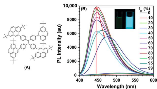
Fig. 17 (A) Molecular structure of TPE-4Py 26 ; (B) PL spectra of TPE-4Py 26 in THF/H 2 O mixtures with different water fractions. Concentration: 10 \mu M; excitation wavelength: 330 nm; inset: photographs of TPE-4Py 26 in THF/H 2 O mixtures ( f_w = 0\% and 90%) taken under illumination by a 365 nm UV lamp. Reproduced from ref. 49.
