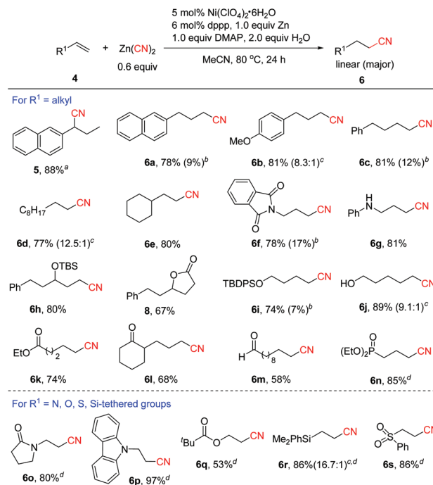
Scheme 3 Scope of aliphatic alkenes. Isolated yields. a 5 mol% \text{NiCl}_2 \cdot 6\text{H}_2\text{O} , 6 mol% Xantphos, 20 mol% Zn, dioxane/ \text{H}_2\text{O} = 50/1 . b The yields of the branched nitrile 7 are shown in parentheses. c Overall yields of 6 and 7 , and the ratio of 6 : 7 is shown in parentheses. d 5 mol% \text{NiCl}_2 \cdot 6\text{H}_2\text{O} , 6 mol% dpfp, 20 mol% Zn and 2.0 equiv. \text{H}_2\text{O} were used in MeCN at 80 °C for 12 h.
