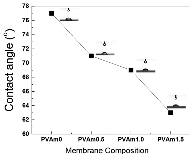
Fig. 8 Effect of PVAm content on the membrane hydrophobicity by contact angle measurement.
