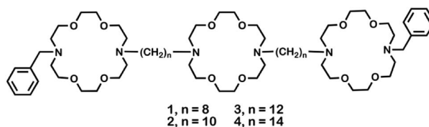
Fig. 1 Structures of hydrapiles studied.
